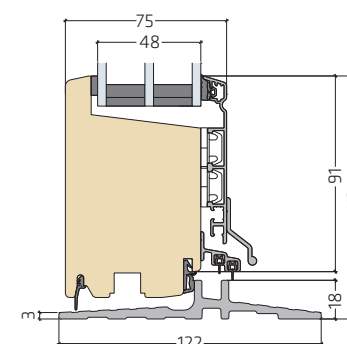
Inward opening entrance door with 18 mm composite threshold
