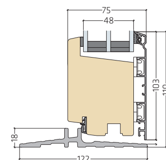
Outward opening entrance door with 18 mm composite threshold
