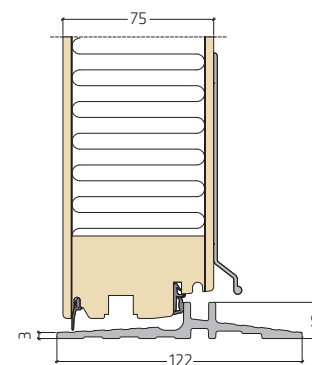
Inward opening entrance door with 18 mm composite threshold
