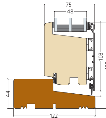
Hardwood threshold for outward opening door
