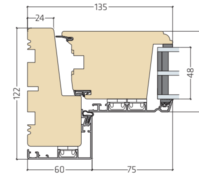
Jamb for inward opening door with triple glazing and profile
