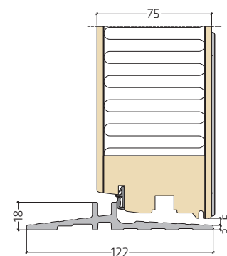
Outward opening entrance door with 18 mm composite threshold
