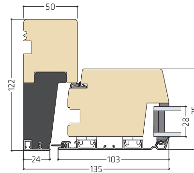
Hardwood threshold for outward opening door
