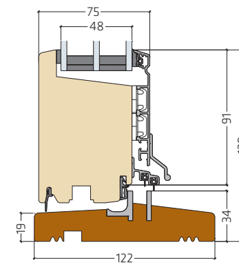
Hardwood threshold for inward opening doors
