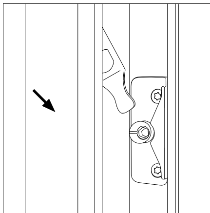
Fig. 5 Adjustment of sash support
