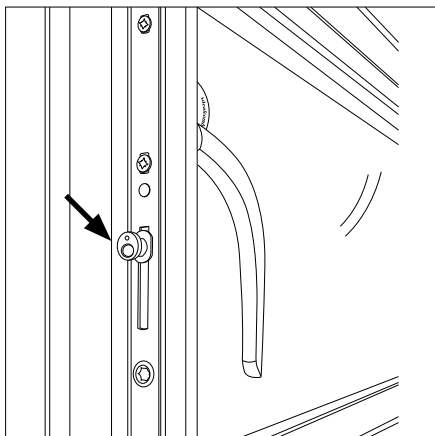
Fig. 3 Adjustment of mushroom bolt
