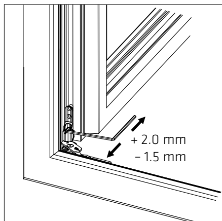
Fig. 2 Lateral adjustment of the sash, bottom
