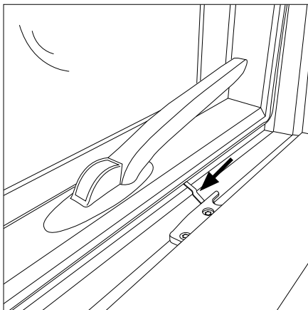
Fig. 6 Ventilation position See page 6
