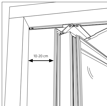
Fig. 5 Cleaning gap
