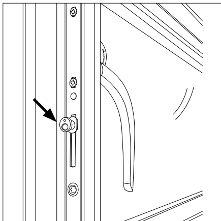
Fig. 5 Adjustment of mushroom bolt
