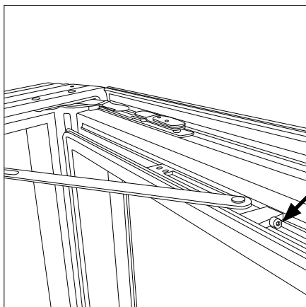
Fig. 8 Adjustment of brake friction
