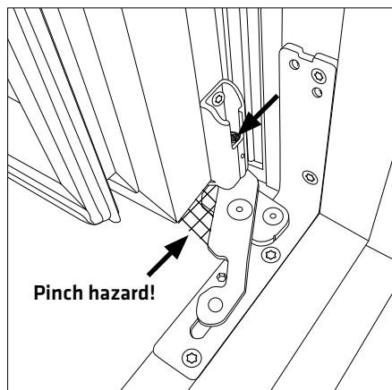
Fig. 1 Height adjustment of the sash
