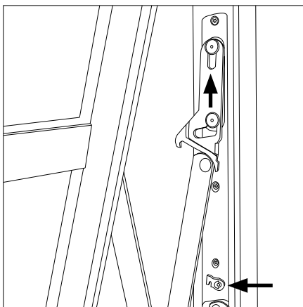
Fig. 2 Safety catch
