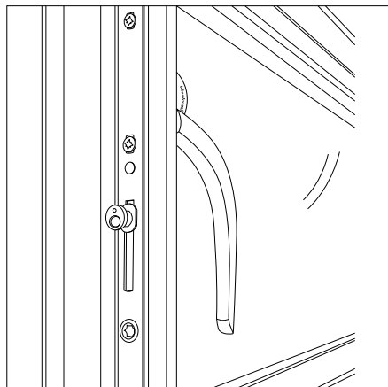
Fig. 4 Adjustment of mushroom bolt
