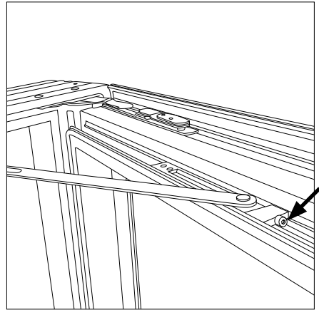
Fig. 6 Adjustment of handle brake
