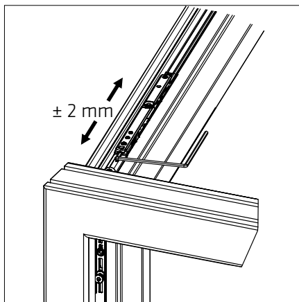
Fig. 3 Lateral adjustment of the sash, head
