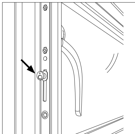
Fig. 1 Adjustment of mushroom bolt
